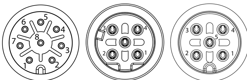
Figure 5: M12 connector pinout, 8-pin A-coded, 4-pin D-coded and 5-pin A-coded.
